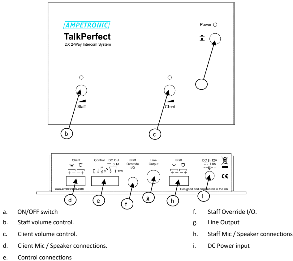
Figure 8 - TalkPerfect™ Connection Diagram
